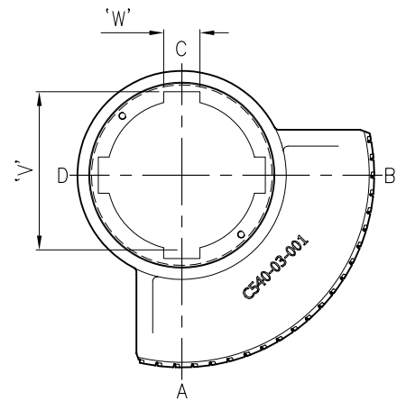
OUTPUT KEYWAY DETAILS SHOWN IN OPEN POSITION
