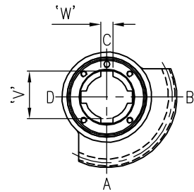
OUTPUT KEYWAY DETAILS SHOWN IN OPEN POSITION
